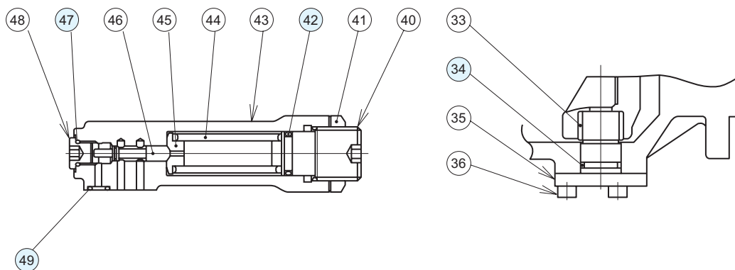
Section A-A Detail of trunnion
